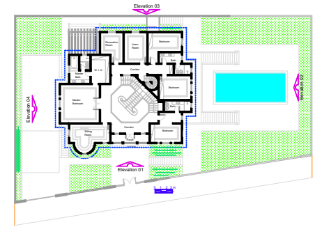
Second Floor Plan A = 214,38 m 2
