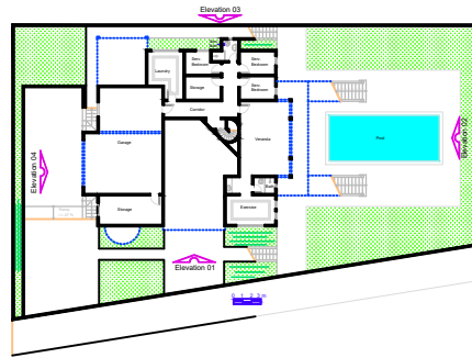
Lower Floor Plan A = 200,83 m 2
